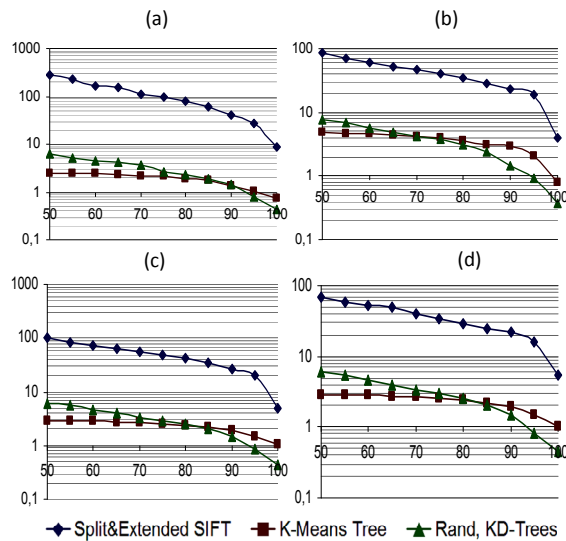
Figure 9: Trade-off between matching speedup (SF) and matching precision for image groups (a) light, (b) viewpoint, (c) rotation, (d) zoom changes.
