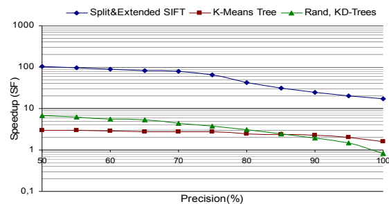
Figure 8: Trade-off between matching speedup and matching precision for real stereo image matching.
