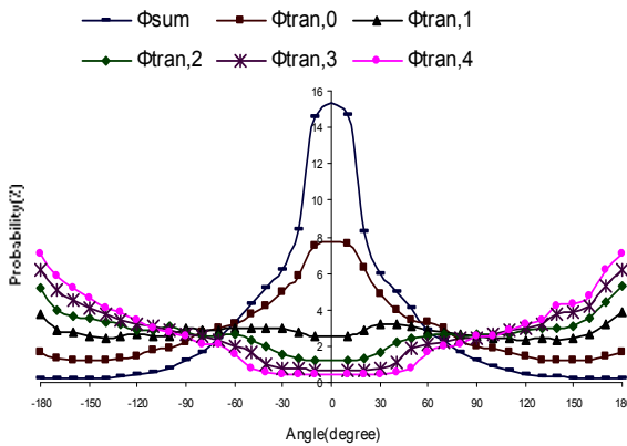
Figure 3: The experimental PDFs of \Phi_{sum} and \Phi_{tran,\kappa} for SIFT features extracted from 600 test images.
