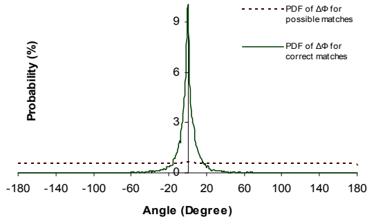
Figure 4: The experimental PDF of the angle difference for the incorrect and the possible matches.
