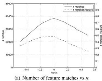
(a) Number of feature matches vs \kappa
