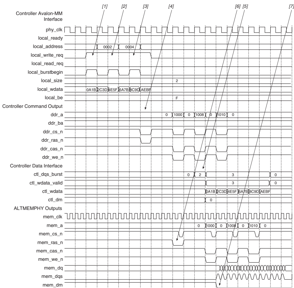
Figure 4-5. Writes
