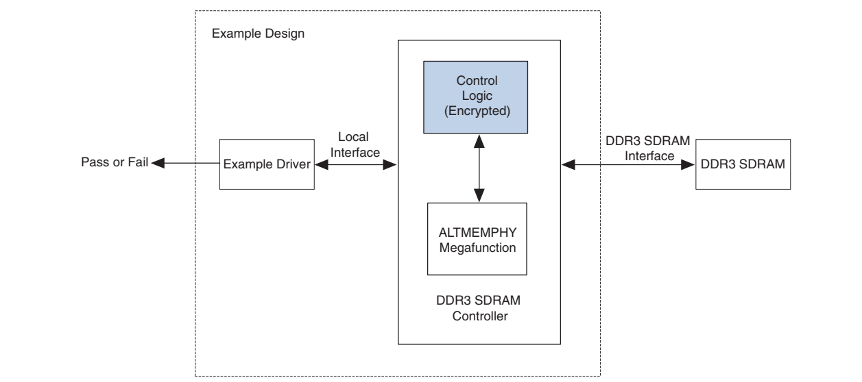
Figure 1-1. System-Level Diagram
