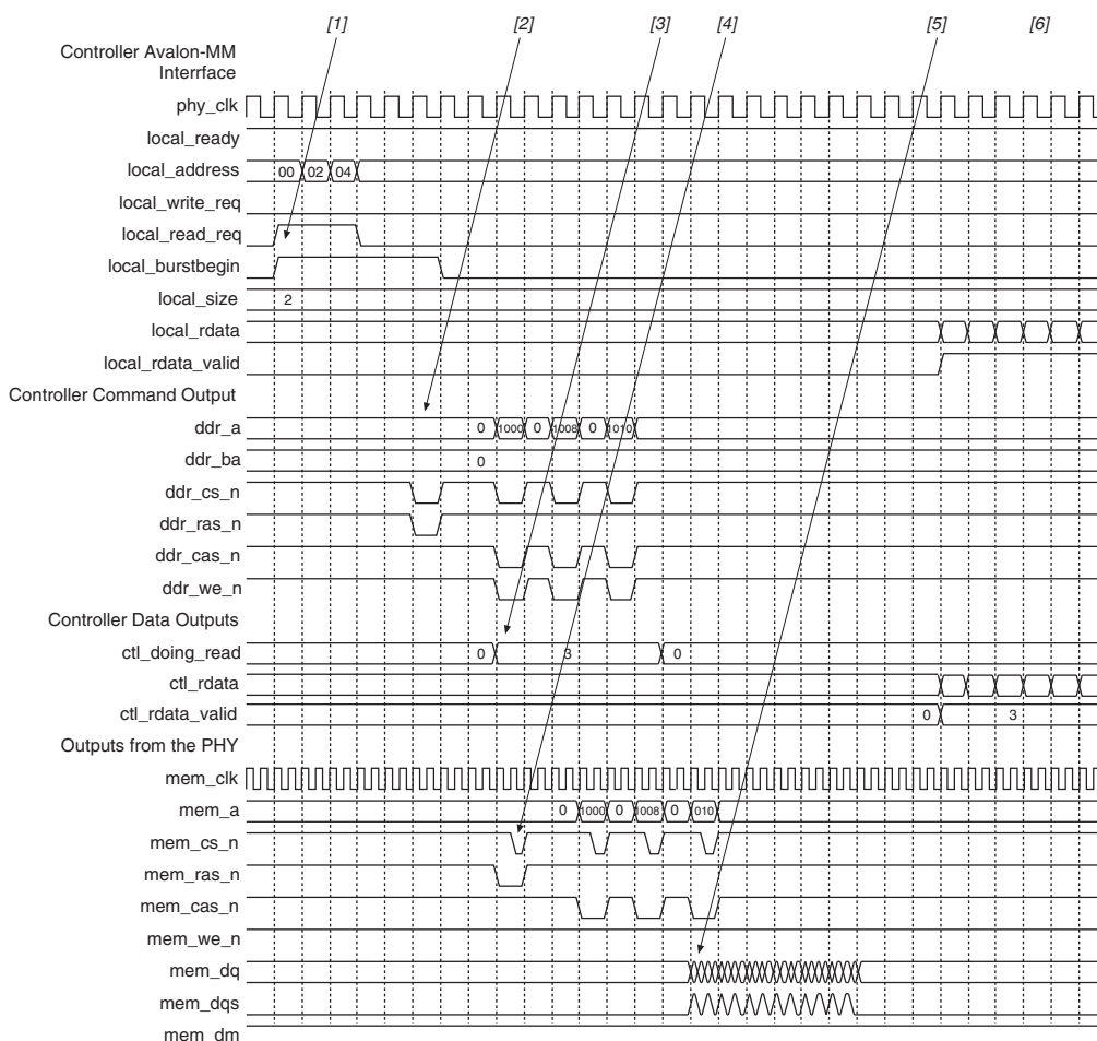
Figure 4-6. Reads
