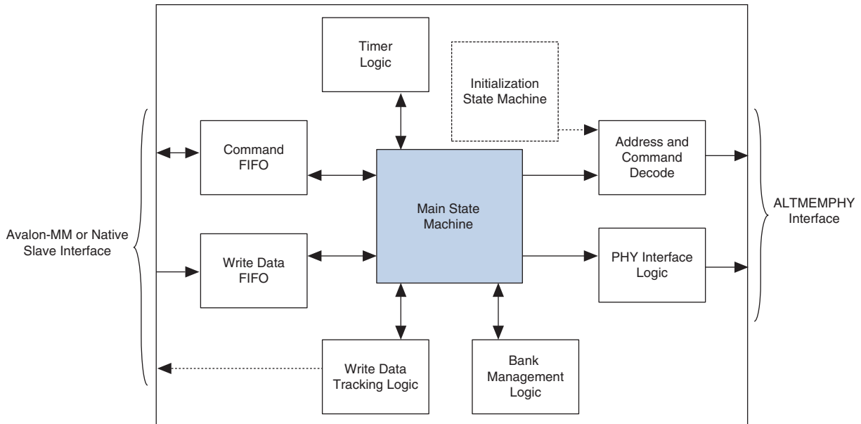
Figure 4-2. DDR3 SDRAM High-Performance Controller Architecture Block Diagram
