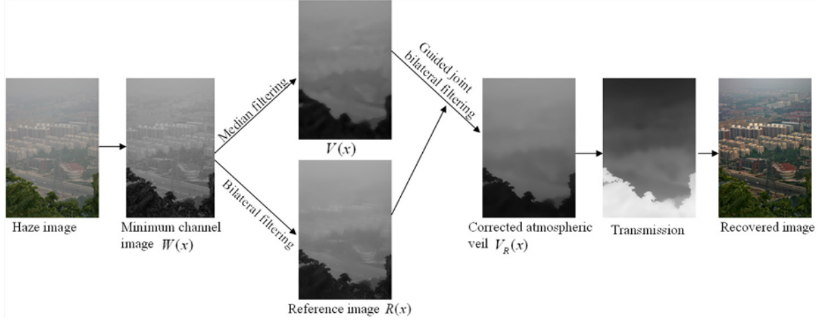
Fig. 2 The flow chart of the proposed method.
