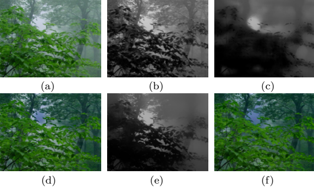
Fig. 5 (a) Input image I , (b) minimal component W of I , (c) atmospheric veil V computed using [18], (d) restored result using the V computed in (c), (e) the atmospheric veil V_R of our method., (f) our final dehazing result.
