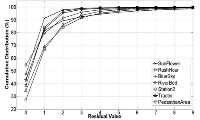
Fig. 6. Cumulative distribution of residuals.
