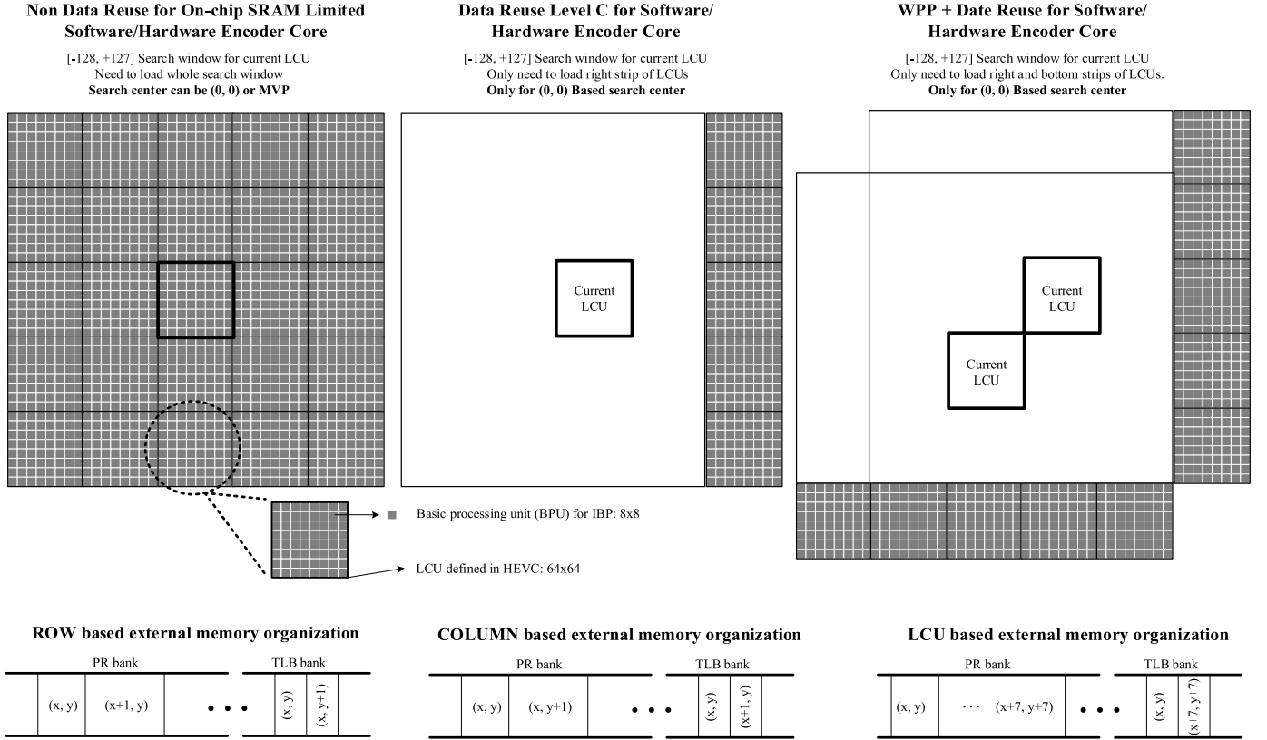
Fig. 8. Data reuse and memory organization for improving DRAM bandwidth utilization.
