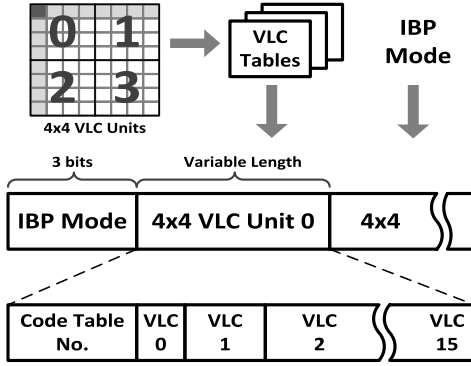
Fig. 7. Small-value optimized variable length coding.
