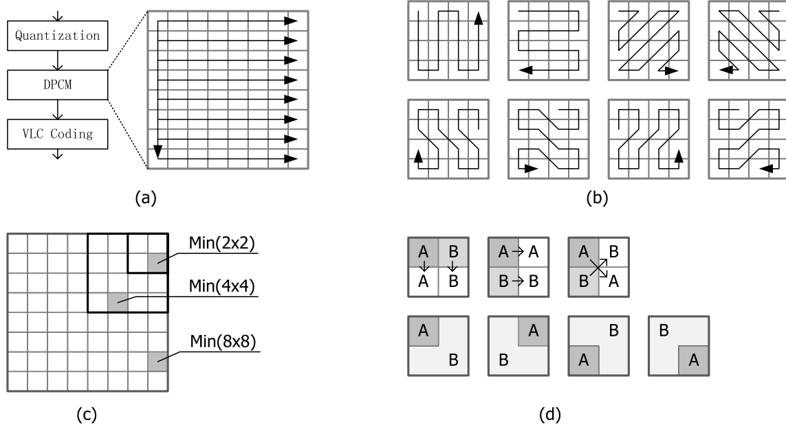
Fig. 2. Existing frame recompression schemes. (a) ADPCM. (b) Intra mode referenced ADPCM. (c) HDM. (d) ERP.
