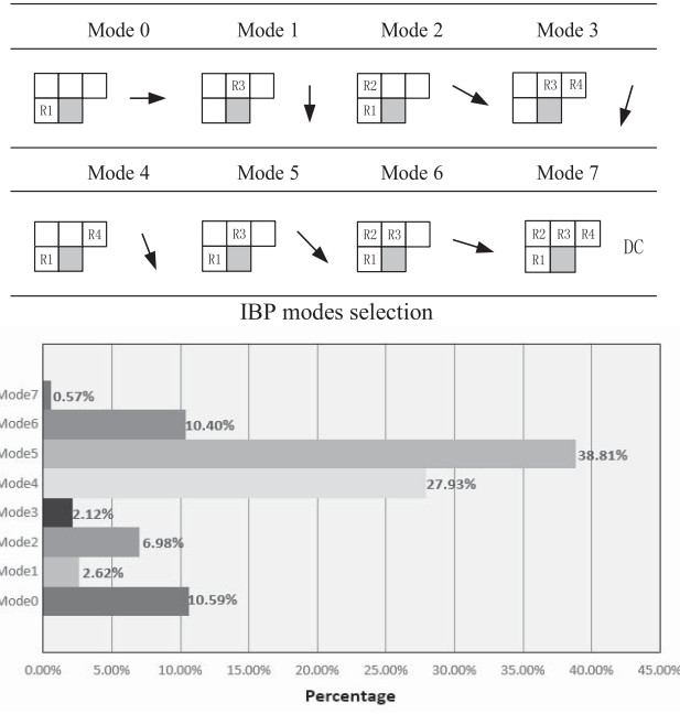
Fig. 9. IBP mode selection and distribution.
