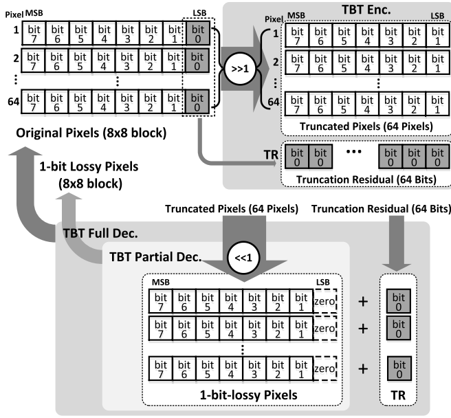
Fig. 4. Tail bit truncation.
