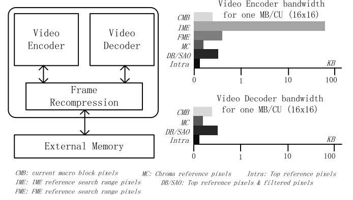
Fig. 1. Frame recompression in video codec.
