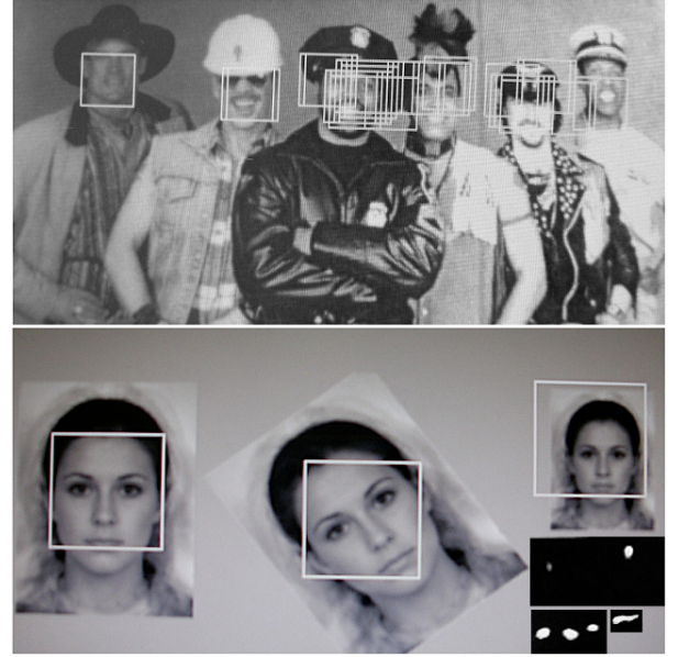
Fig. 4. up: output of the system without non maximum suppression; down: with NMS; bottom corner: output maps for three different scales.
